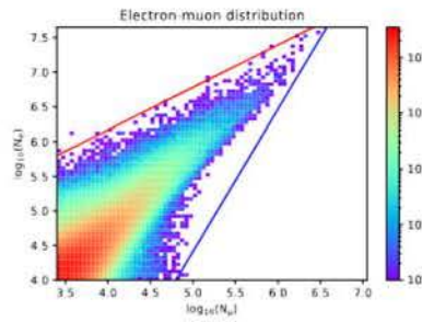
Figure 3: Muon to electron distribution of the KASCADE data sample with an upper and lower line associated with the expected primary mass. The upper line (red) represents light particles and the lower line (blue) represents heavy particles.
