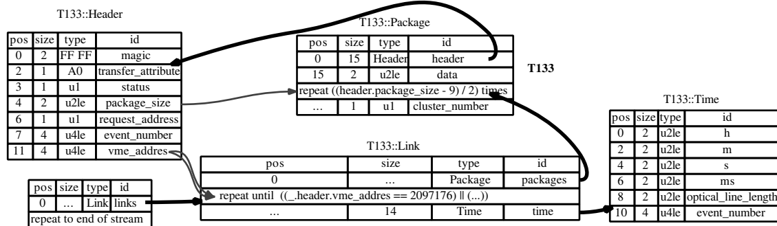
Figure 5. Tunka-133 file format specification presented in Kaitai Struct.
